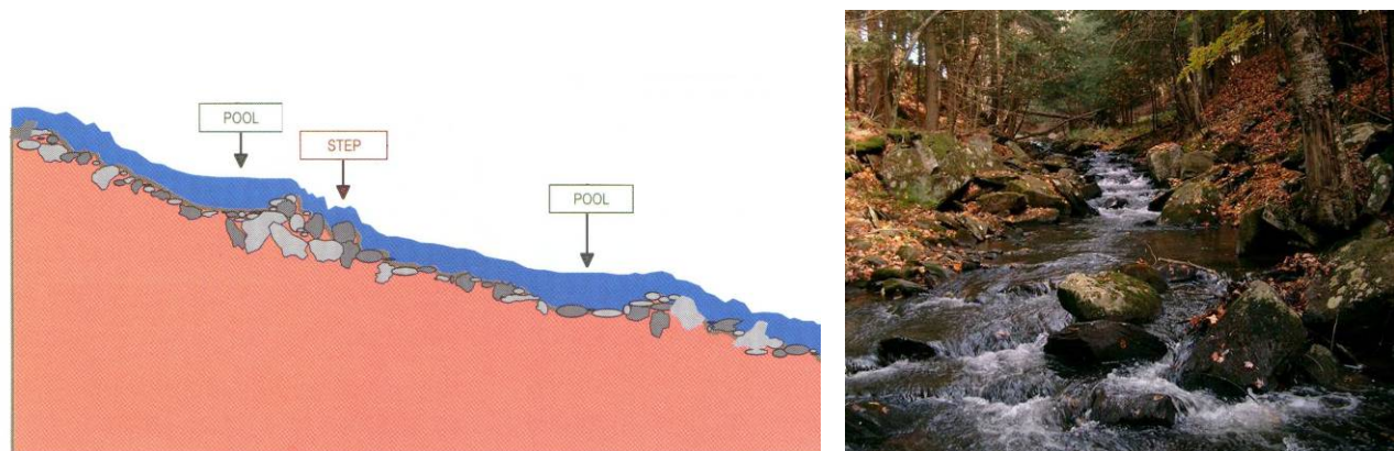
Figure 2.9 Typical Step-Pool Sequence (After Rosgen, 1996)
