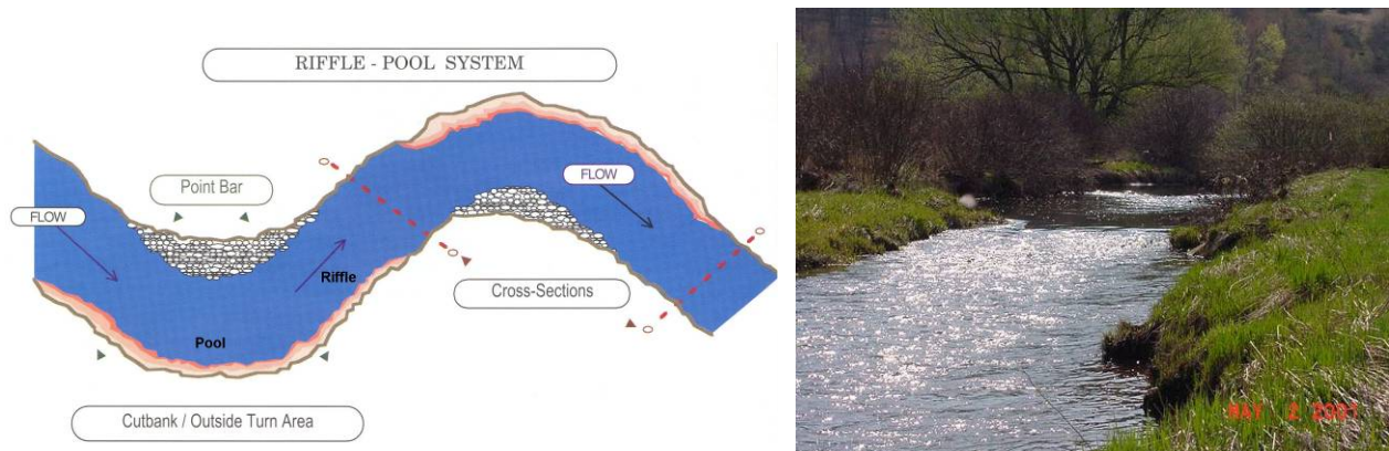
Figure 2.8 Typical Riffle-Pool Sequence (Rosgen, 1996)
